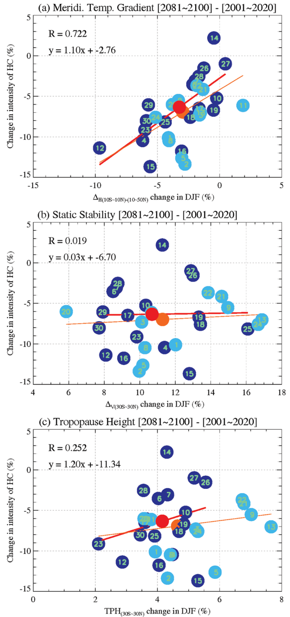
Fig. 2. Changes in the HC strength (%) against changes in (a) meridional potential temperature gradient measured as \Delta_H = \frac{\theta_{[10S-10N]} - \theta_{[10N-50N]}}{\theta_0} , (b) tropical static stability \Delta_S , and (c) subtropical tropopause height during DJF for good models (dark dots). Linear correlation coefficients and regression equations for good models are shown in the plot (i.e., sky blue dots are excluded in the calculation of the statistics). Red line shows a regression line for good models and orange line for all models.
