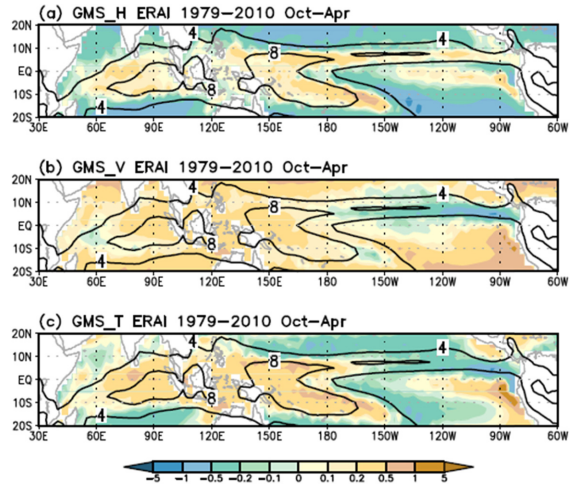
Fig. 2. Climatological mean distribution of (a) the horizontal GMS, (b) the vertical GMS, and (c) the total GMS. Thick solid line denotes October-April climatological mean precipitation (units: \text{mm day}^{-1} ).
