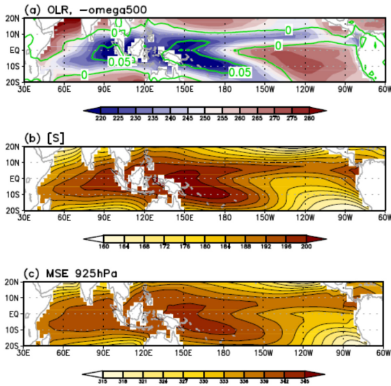
Fig. 1. Climatological mean distribution of (a) outgoing longwave radiation (shading, units: W m^{-2} ) and -\omega at 500 hPa (green contour, units: Pa s^{-1} ), (b) the column-integrated moist entropy (units: W m^{-2} ), and (c) the moist static energy at 925 hPa (units: 10^3 J kg^{-1} ).
