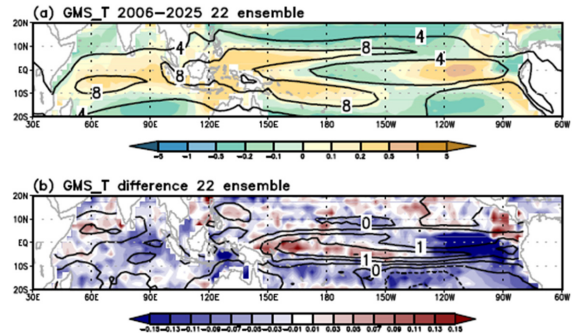
Fig. 6. Climatological mean distribution for 22 models ensemble of (a) the total GMS (shading) and precipitation (contour, units: mm day -1 ) for 2006~2025, and (b) the difference between 2081~2100 and 2006~2025 for the total GMS (shading) and precipitation (contour, units: mm day -1 ).
