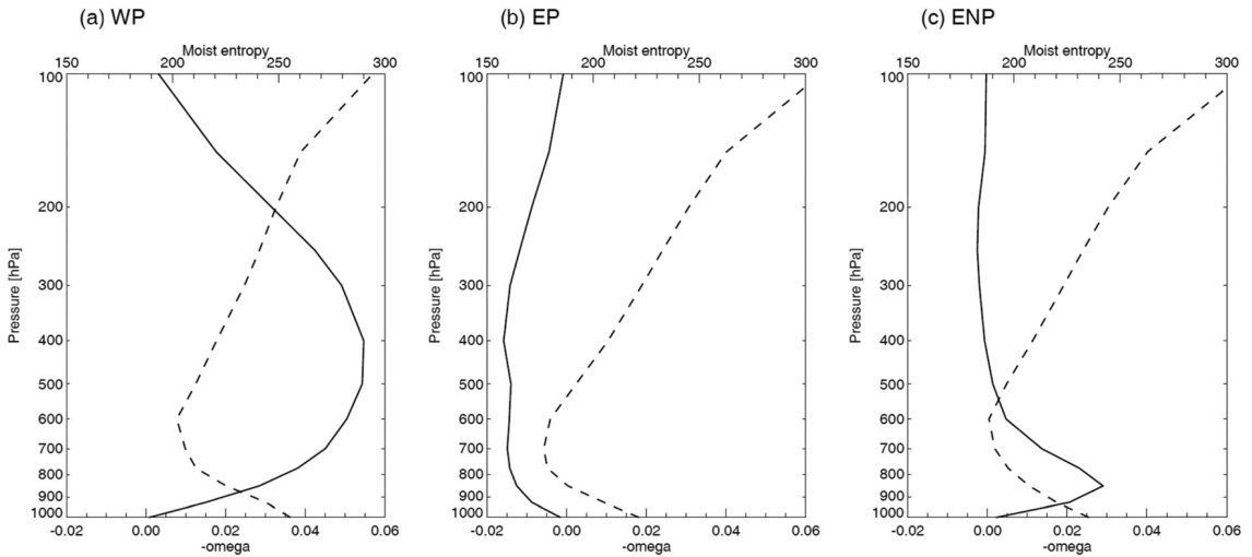
Fig. 5. Vertical profile of the moist entropy (dashed lines, units: J K^{-1} kg^{-1} ) and -\omega (solid lines, units: Pa s^{-1} ) averaged over (a) the western Pacific ( 5^{\circ}S\sim 5^{\circ}N, 140\sim 170^{\circ}E ), (b) the eastern Pacific ( 7.5^{\circ}S\sim 0, 230\sim 270^{\circ}E ), and (c) the eastern Pacific ITCZ ( 0\sim 10^{\circ}N, 230\sim 270^{\circ}E ).
